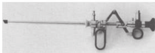
▲ Figure 8-6. Transurethral resectoscope. Left: Continuous-flow sheath, standard sheath, working element with cutting loop, telescope. Right: Instrument assembled.
