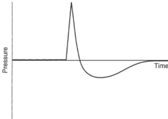
▲ Figure 17-17. Graphical representation of a shockwave. Vertical axis (ordinate) represents pressure and horizontal axis (abscissa) represents time.
